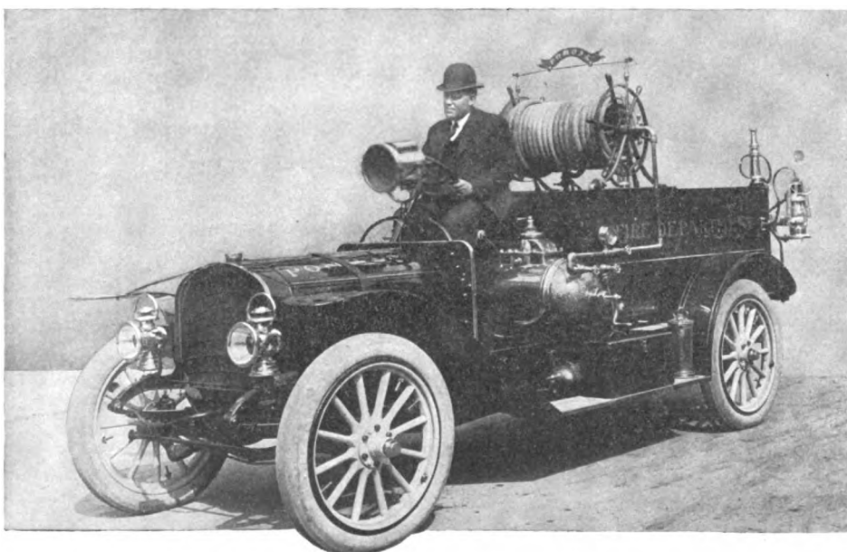
Rambler Chassis with Home-built Body in Service of Pomona, Cal., Fire Department
